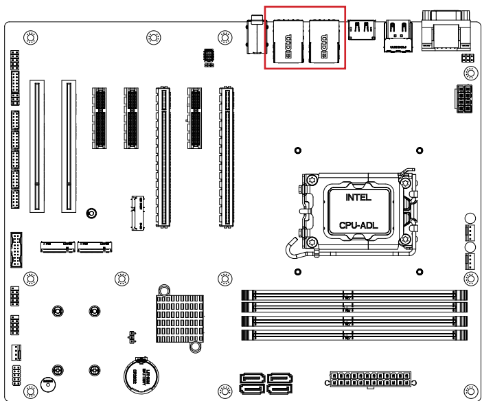
USB & LAN Connector
