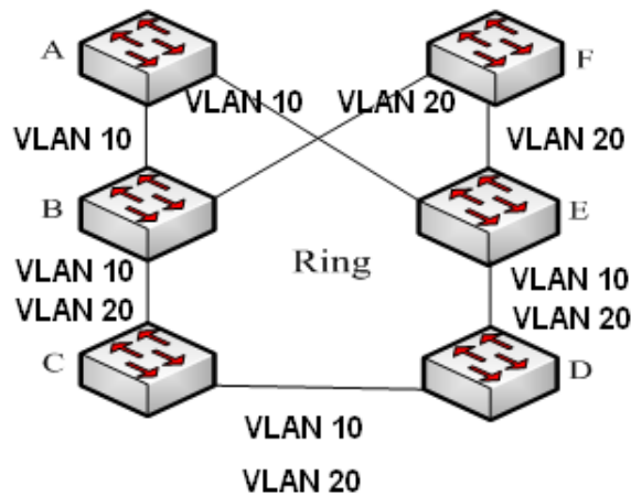
Figure 195 DT-Ring-VLAN
