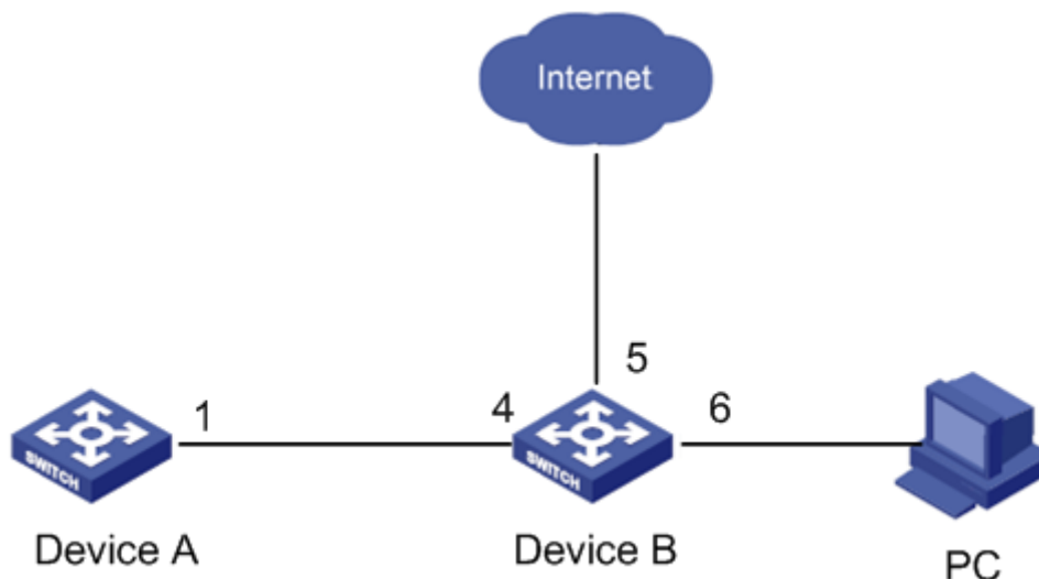
Figure 192 GVRP Configuration Example
