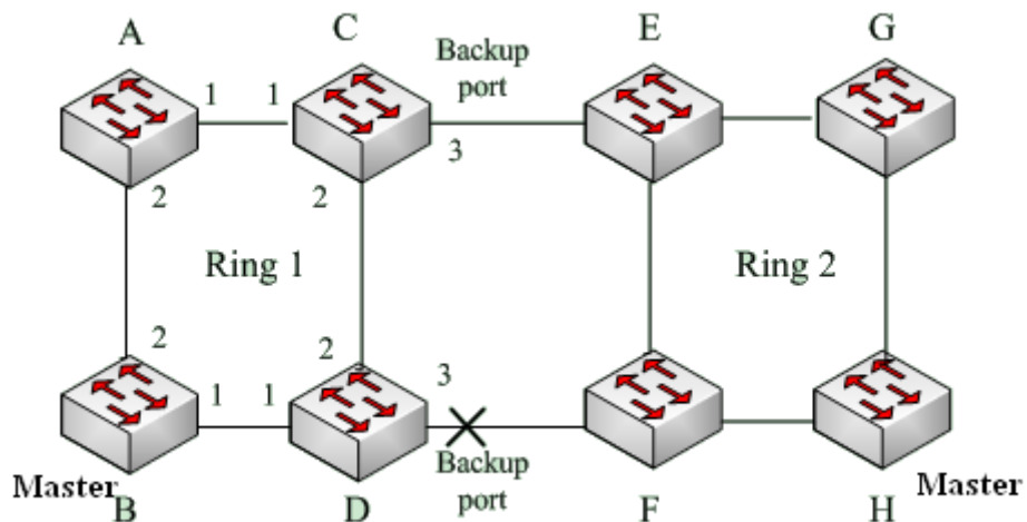
Figure 196 DT-Ring+ Topology
