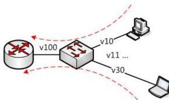
Figure 186 PVLAN Application
