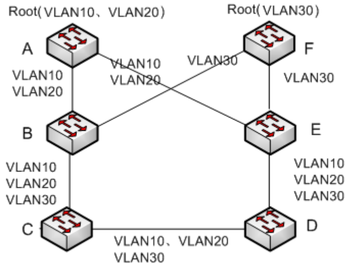
Figure 203 DRP-VLAN-Based
