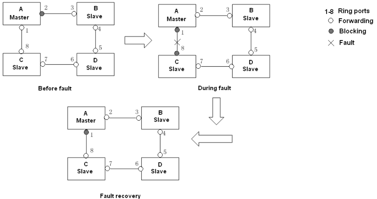
Figure 194 DT-Ring Link Fault
