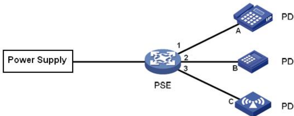
Figure 172 POE Power Supply System
