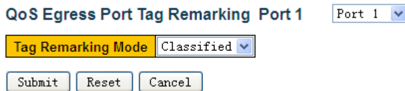
Figure 58 Configure 802.1p Remarking Mode to Classified
