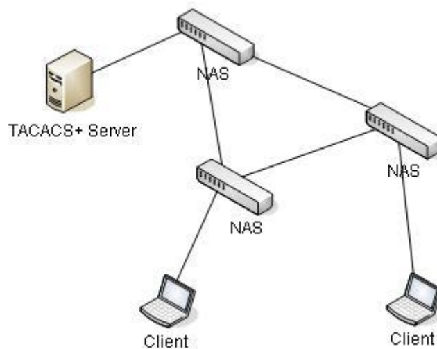
Figure 125 TACACS+ Structure
