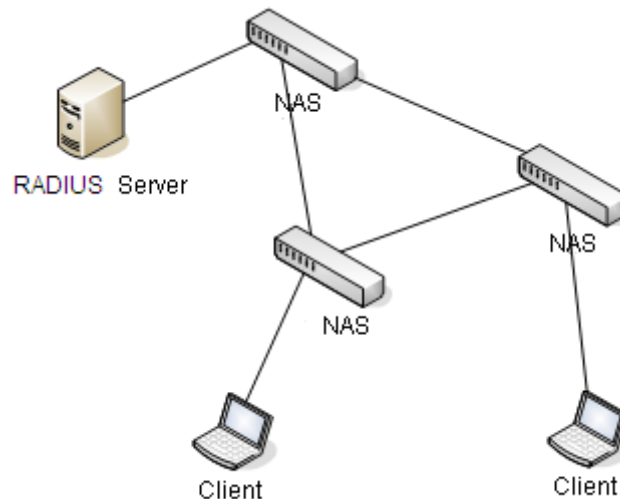
Figure 129 RADIUS Structure
