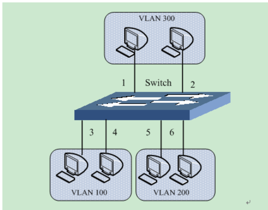
Figure 187 PVLAN Configuration Example
