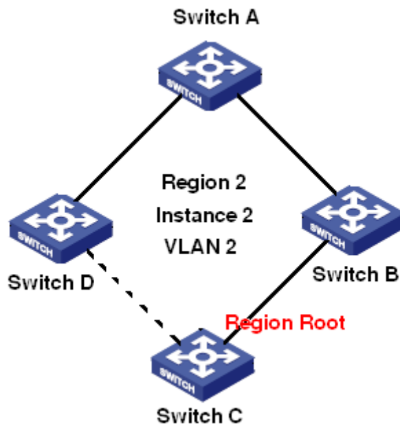
Figure 220 VLAN2 Mapping to Instance 2
