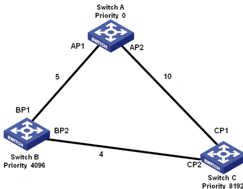
Figure 215 RSTP Configuration Example
