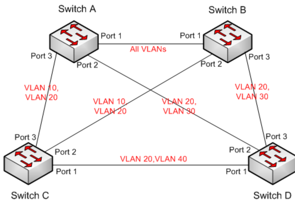
Figure 231 MSTP Typical Configuration Example
