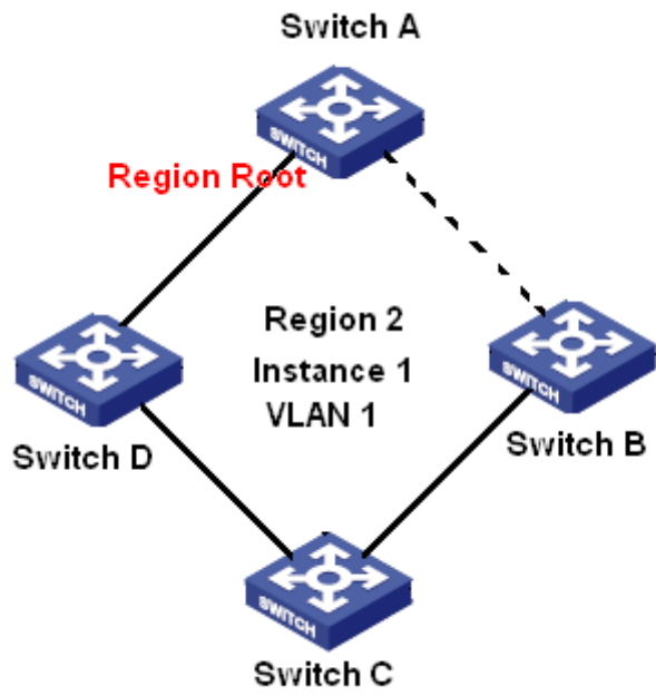
Figure 219 VLAN 1 Mapping to Instance 1
