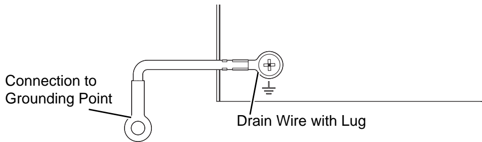
Figure 2.17 Grounding Connection
