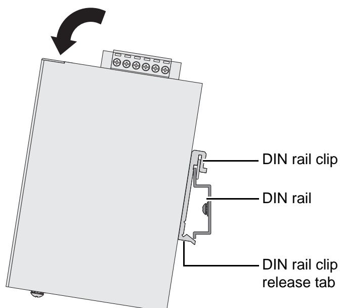
Figure 2.1 Installing the DIN-Rail Mounting Kit
