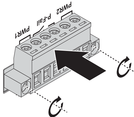
Figure 2.24 Securing a Terminal Block to a Receptor
