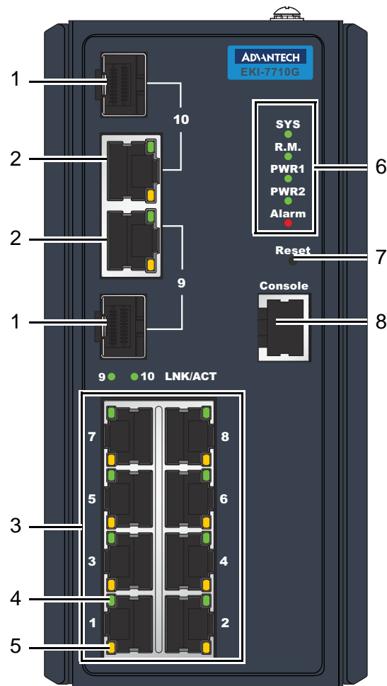
Figure 1.1 Front View
